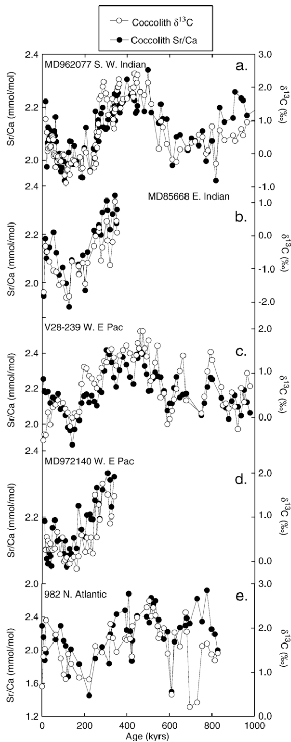
Fig. 3. \delta^{13}\text{C} (open circles) and Sr/Ca (closed circles) measured in the CF from global ocean cores: (a) MD962077 S. W. Indian Ocean, (b) MD 85668 Equatorial Indian Ocean, (c) V28–239, (d) MD972140 west Equatorial Pacific, (e) ODP 982 N. Atlantic.
